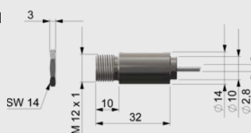
Sensing head (built-in CF lense)
